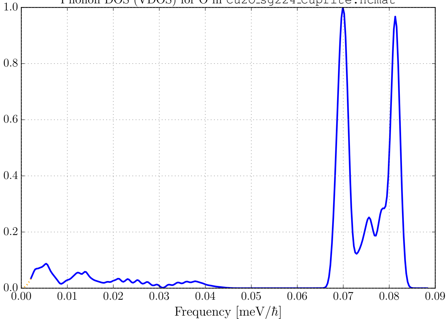
Phonon DOS (VDOS) for O in Cu2O_sg224_Cuprite.ncmat
