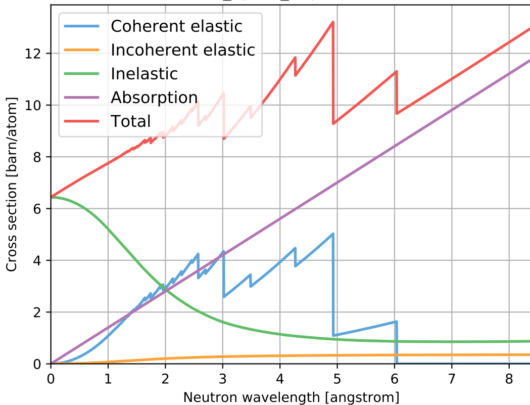
Cu2O_sg224_Cuprite.ncmat
