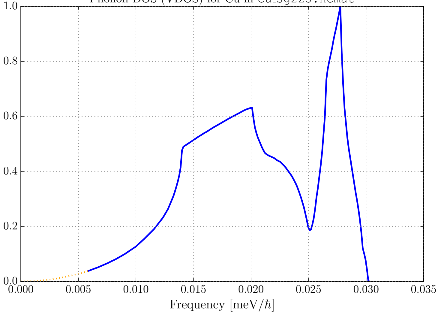
Phonon DOS (VDOS) for Cu in Cu_sg225.ncmat
