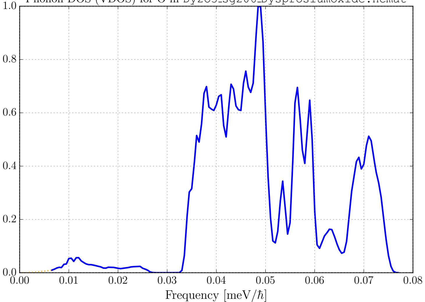
Phonon DOS (VDOS) for O in Dy2O3_sg206_DysprosiumOxide.ncmat
