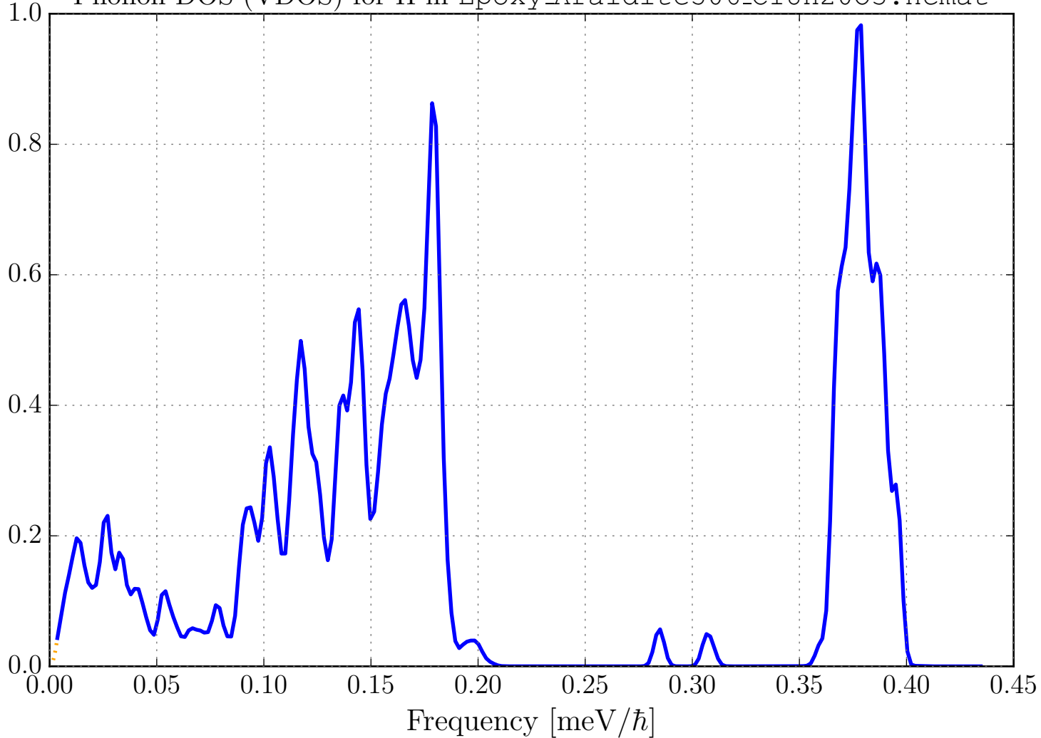
Phonon DOS (VDOS) for H in Epoxy_Araldite506_C18H20O3.ncmat
