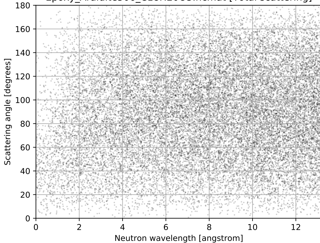
Epoxy_Araldite506_C18H20O3.ncmat [Total scattering]
