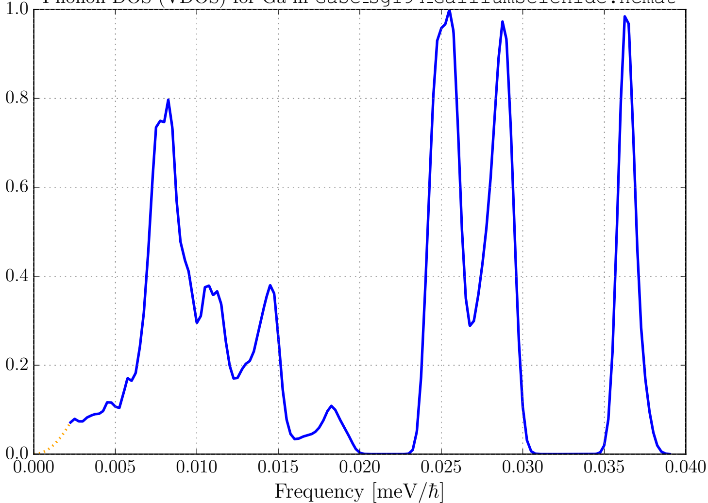
Phonon DOS (VDOS) for Ga in GaSe_sg194_GalliumSelenide.ncmat
