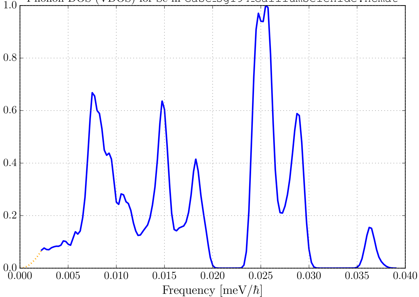
Phonon DOS (VDOS) for Se in GaSe_sg194_GalliumSelenide.ncmat
