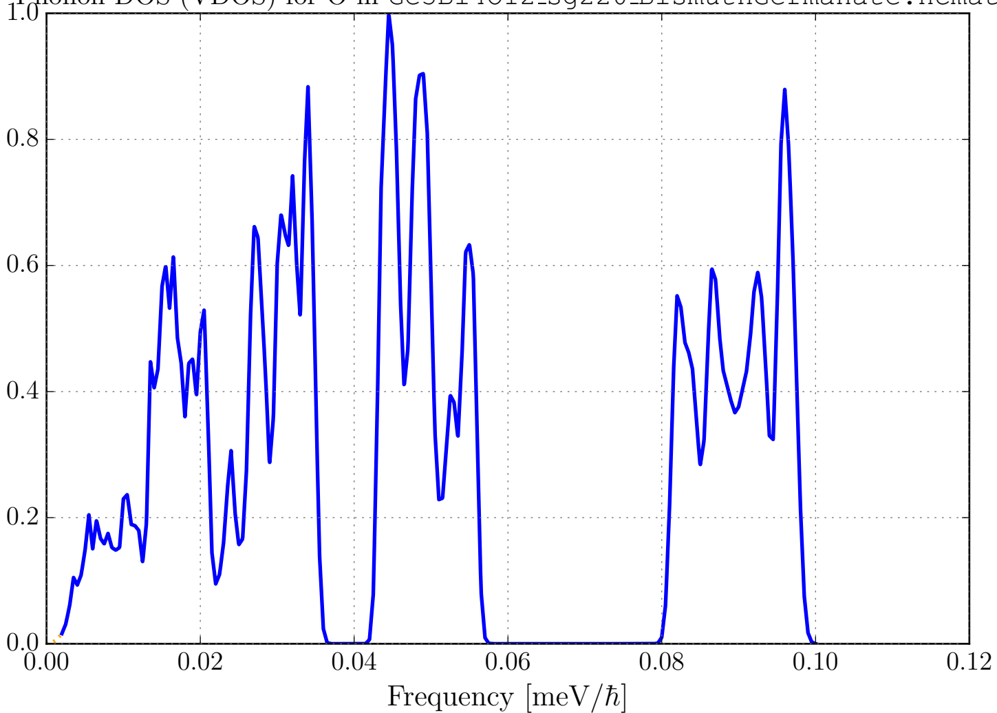
Phonon DOS (VDOS) for O in Ge 3 Bi 4 O 12 _sg220_BismuthGermanate.ncmat
