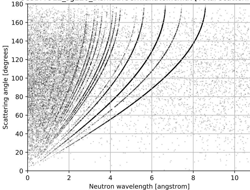
Ge3Bi4O12_sg220_BismuthGermanate.ncmat [Total scattering]
