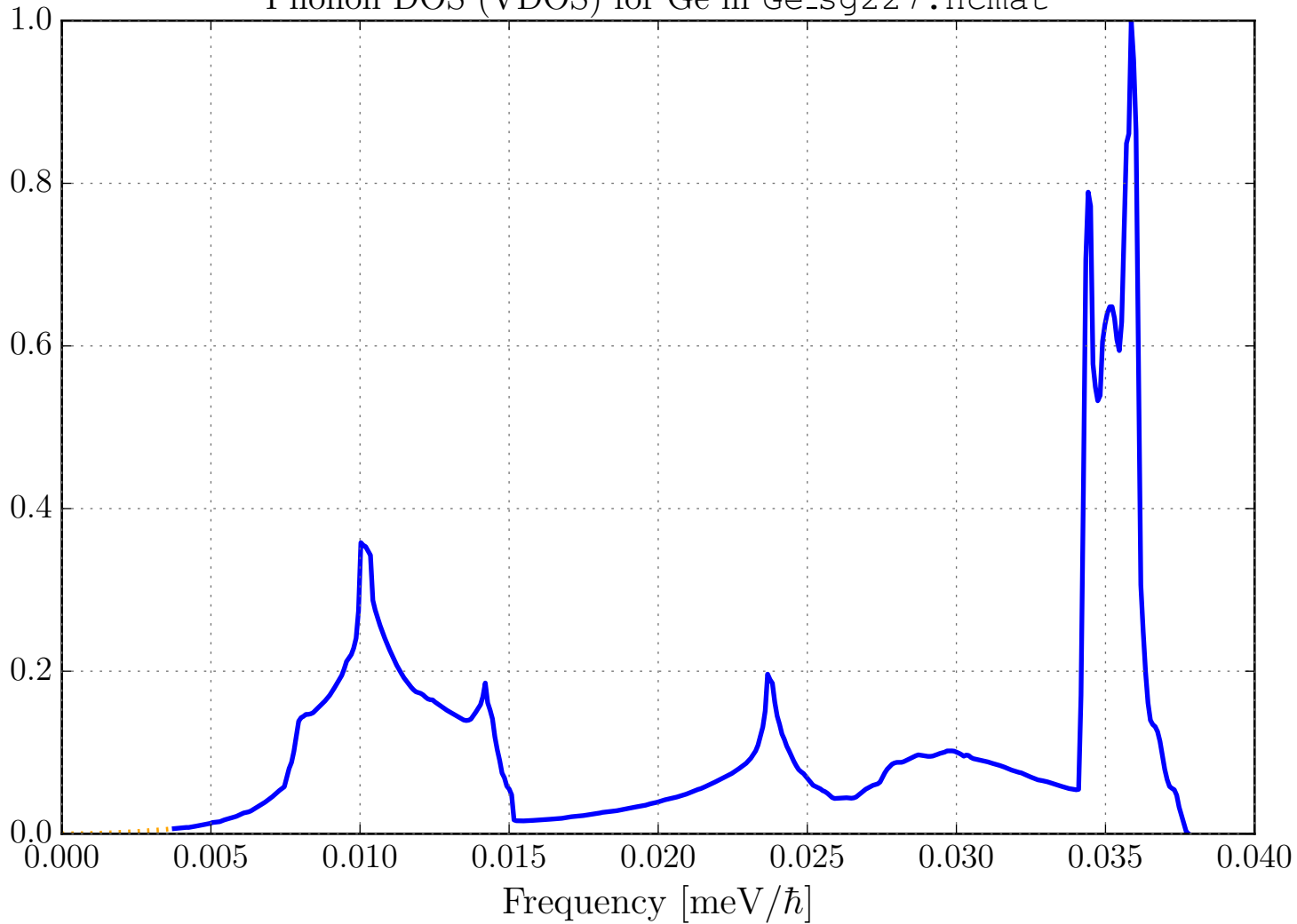
Phonon DOS (VDOS) for Ge in Ge_sg227.ncmat
