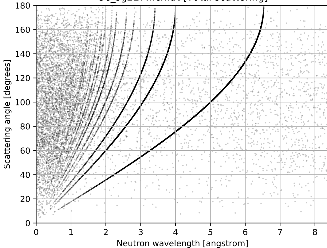
Ge_sg227.ncmat [Total scattering]
