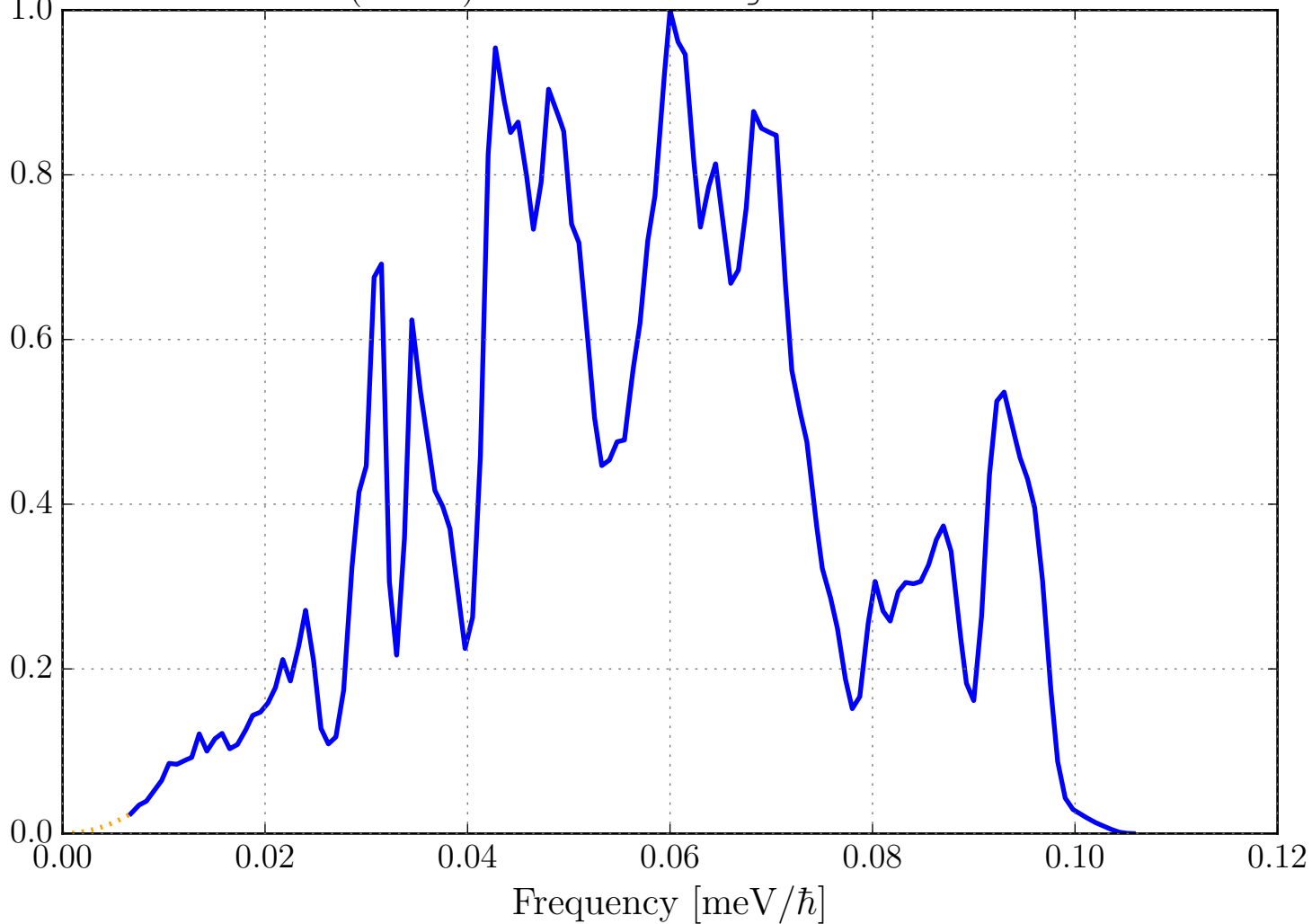
Phonon DOS (VDOS) for O in HfO2_sg14_HafniumOxide.ncmat
