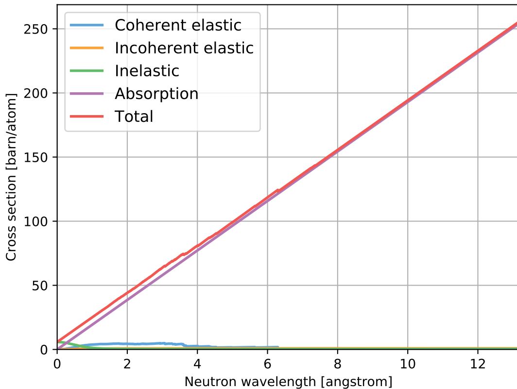
HfO2_sg14_HafniumOxide.ncmat [dcutoff=0.2]
