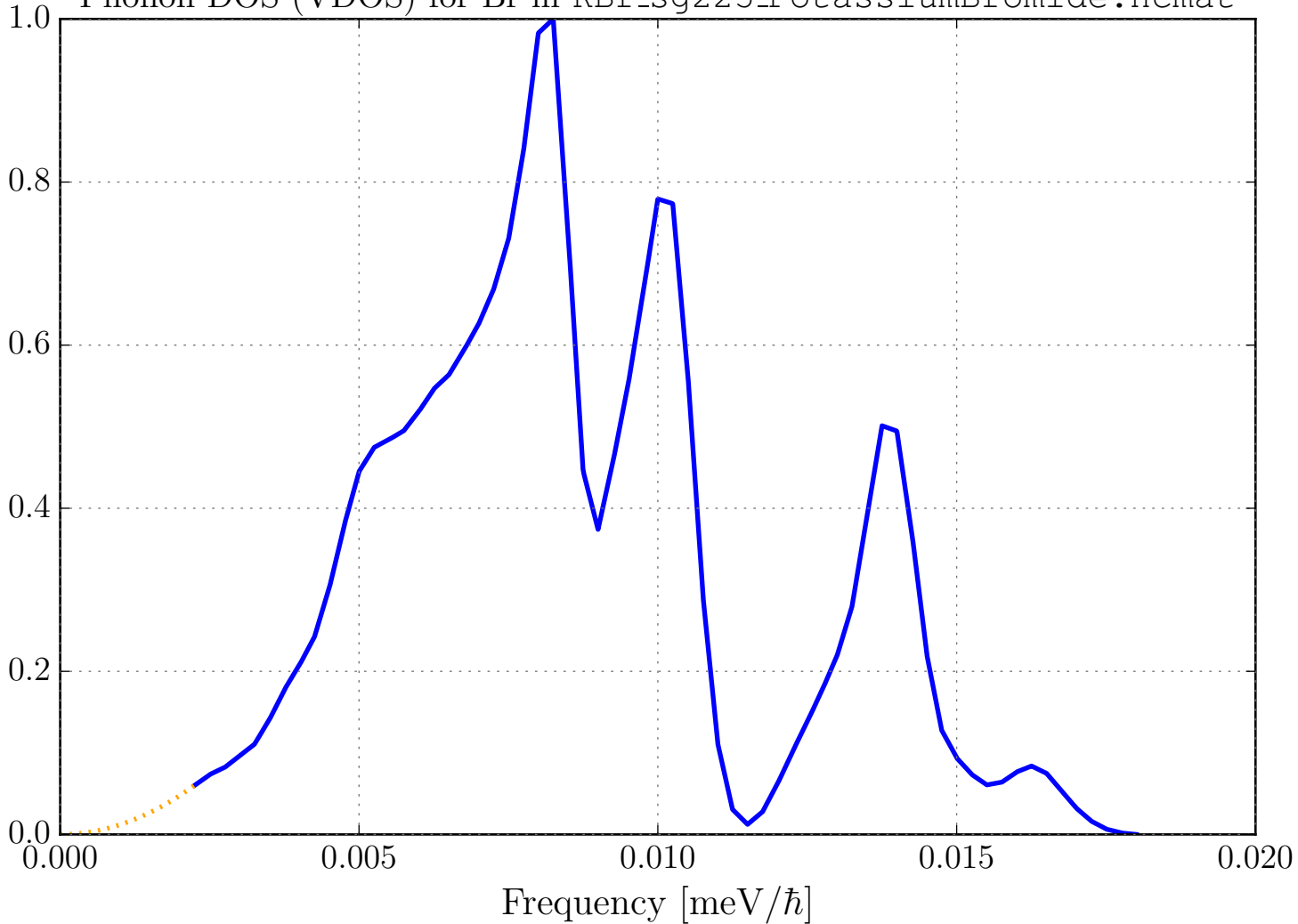
Phonon DOS (VDOS) for Br in KBr_sg225_PotassiumBromide.ncmat
