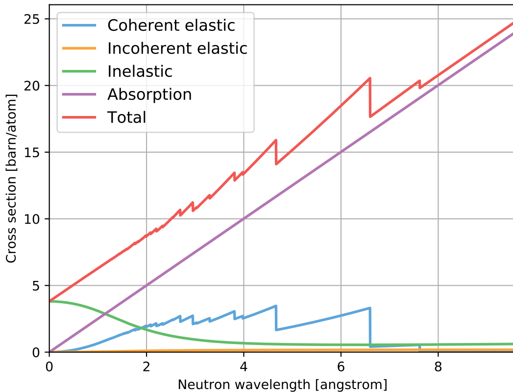
KBr_sg225_PotassiumBromide.ncmat
