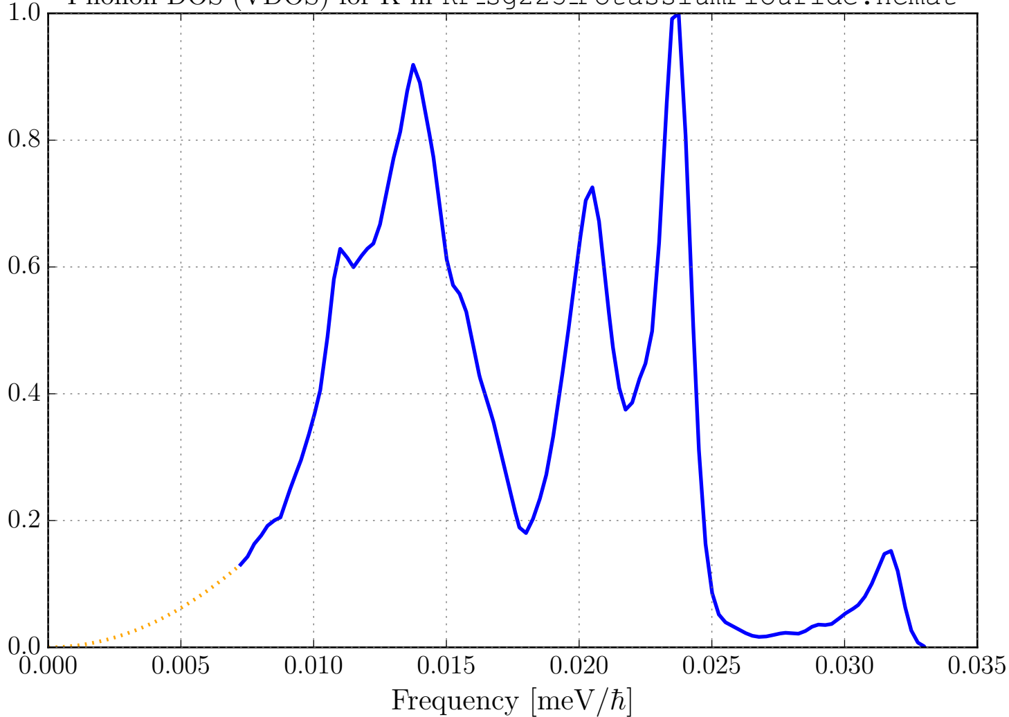
Phonon DOS (VDOS) for K in KF_sg225_PotassiumFlouride.ncmat
