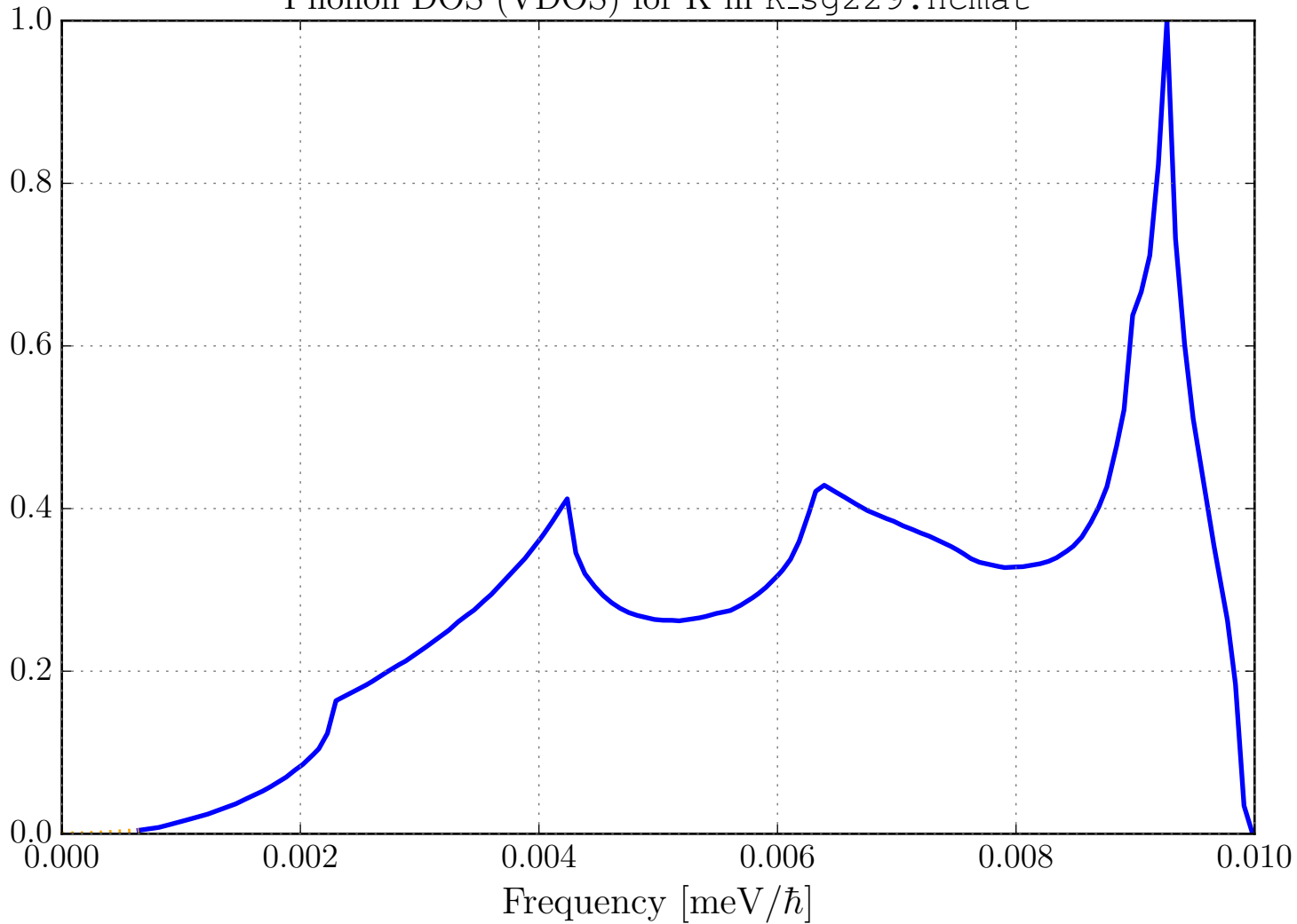
Phonon DOS (VDOS) for K in K_sg229.ncmat
