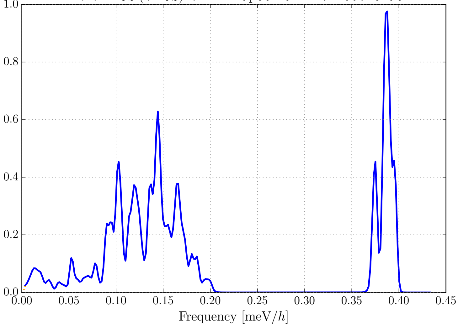
Phonon DOS (VDOS) for H in Kapt on_C22H10N2O5.ncmat
