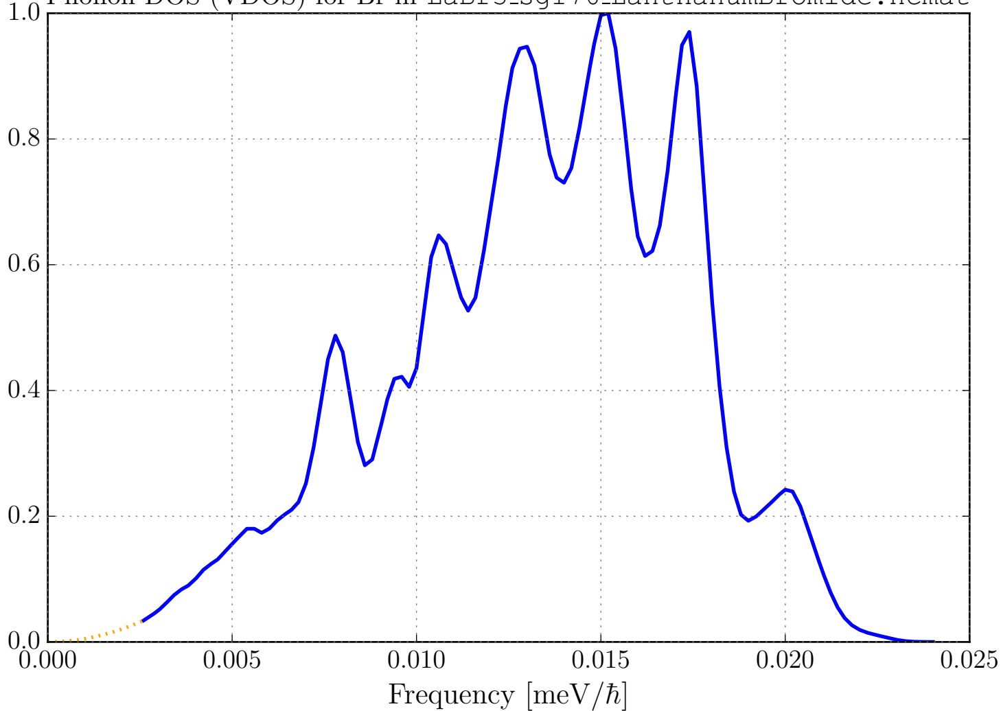
Phonon DOS (VDOS) for Br in LaBr3_sg176_LanthanumBromide.ncmat
