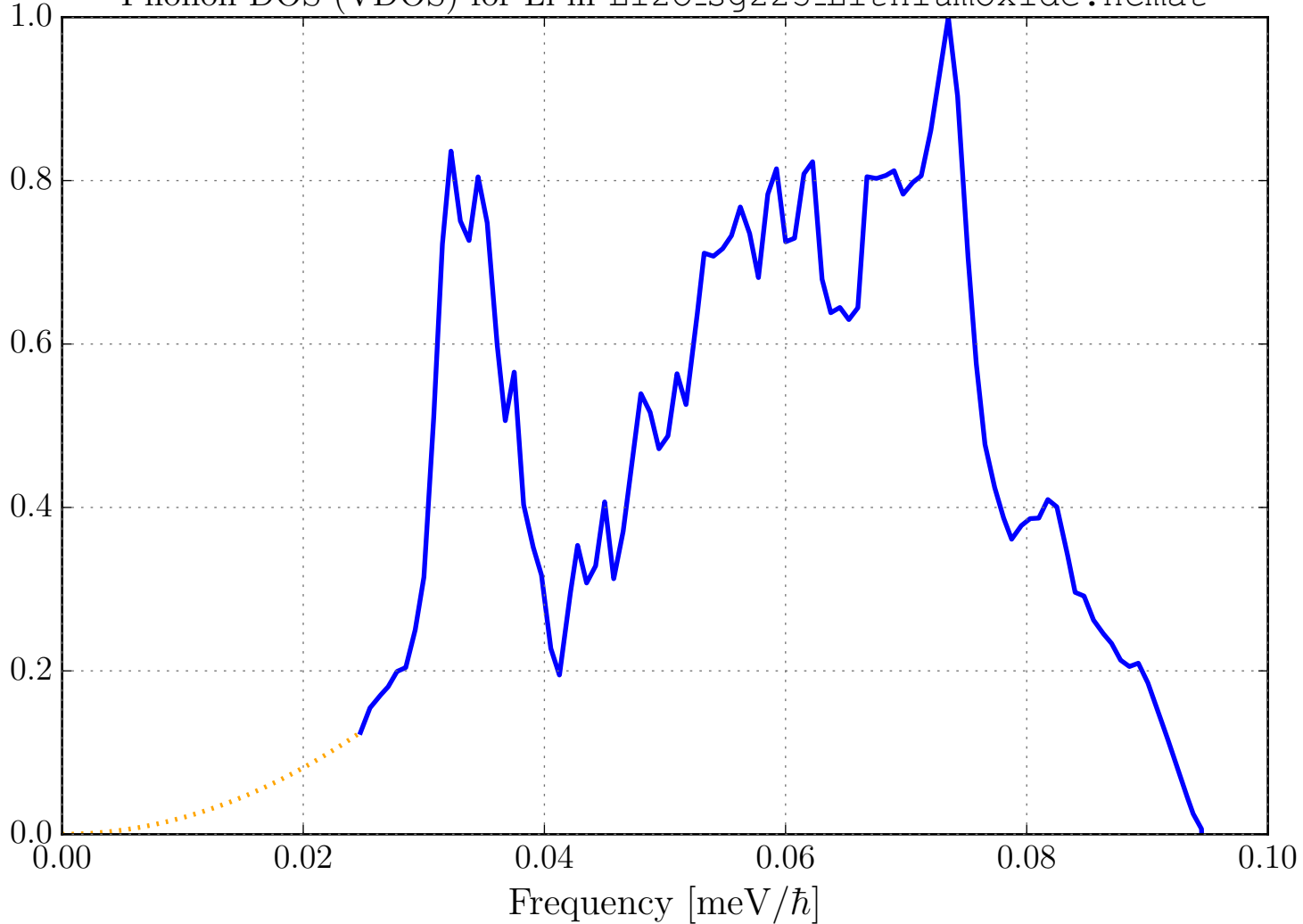
Phonon DOS (VDOS) for Li in Li2O_sg225_LithiumOxide.ncmat
