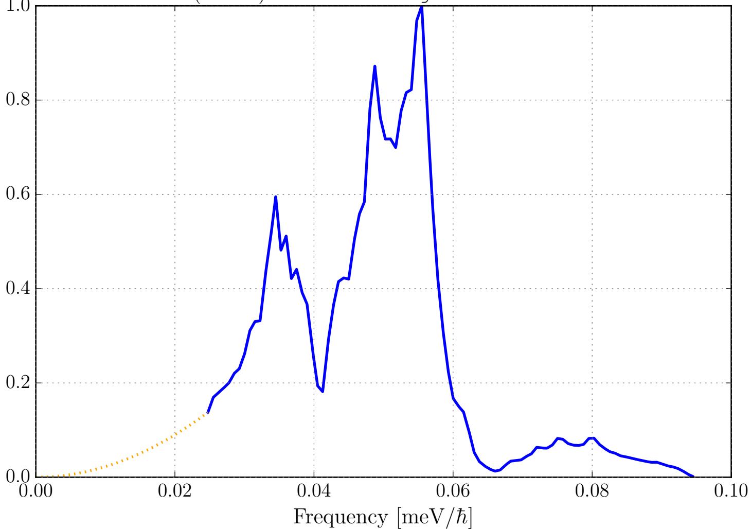
Phonon DOS (VDOS) for O in Li2O_sg225_LithiumOxide.ncmat
