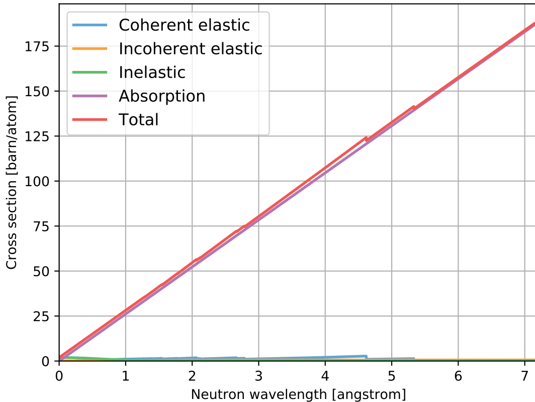
Li2O_sg225_LithiumOxide.ncmat
