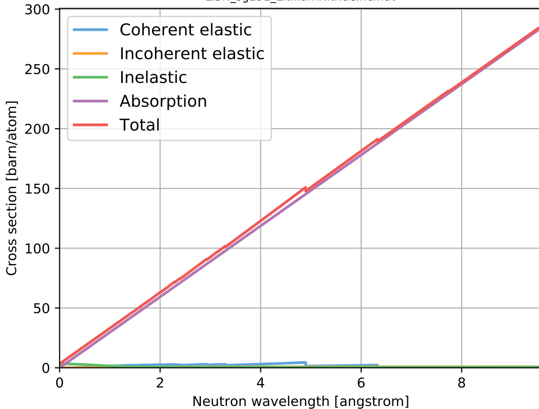
Li3N_sg191_LithiumNitride.ncmat
