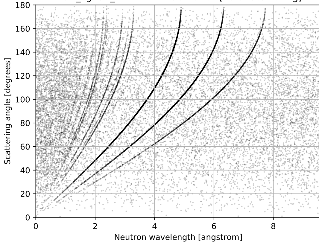
Li3N_sg191_LithiumNitride.ncmat [Total scattering]
