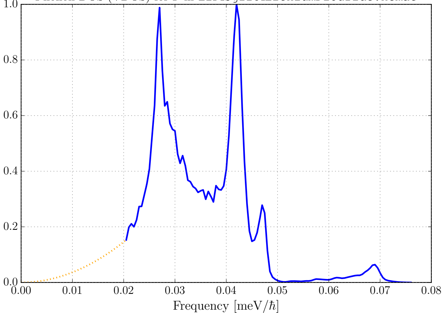
Phonon DOS (VDOS) for F in LiF_sg225_LithiumFlouride.ncmat
