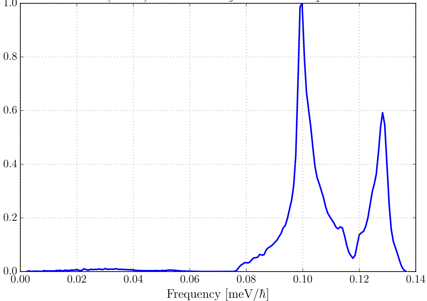
Phonon DOS (VDOS) for H in LiH_sg225_LithiumHydride.ncmat
