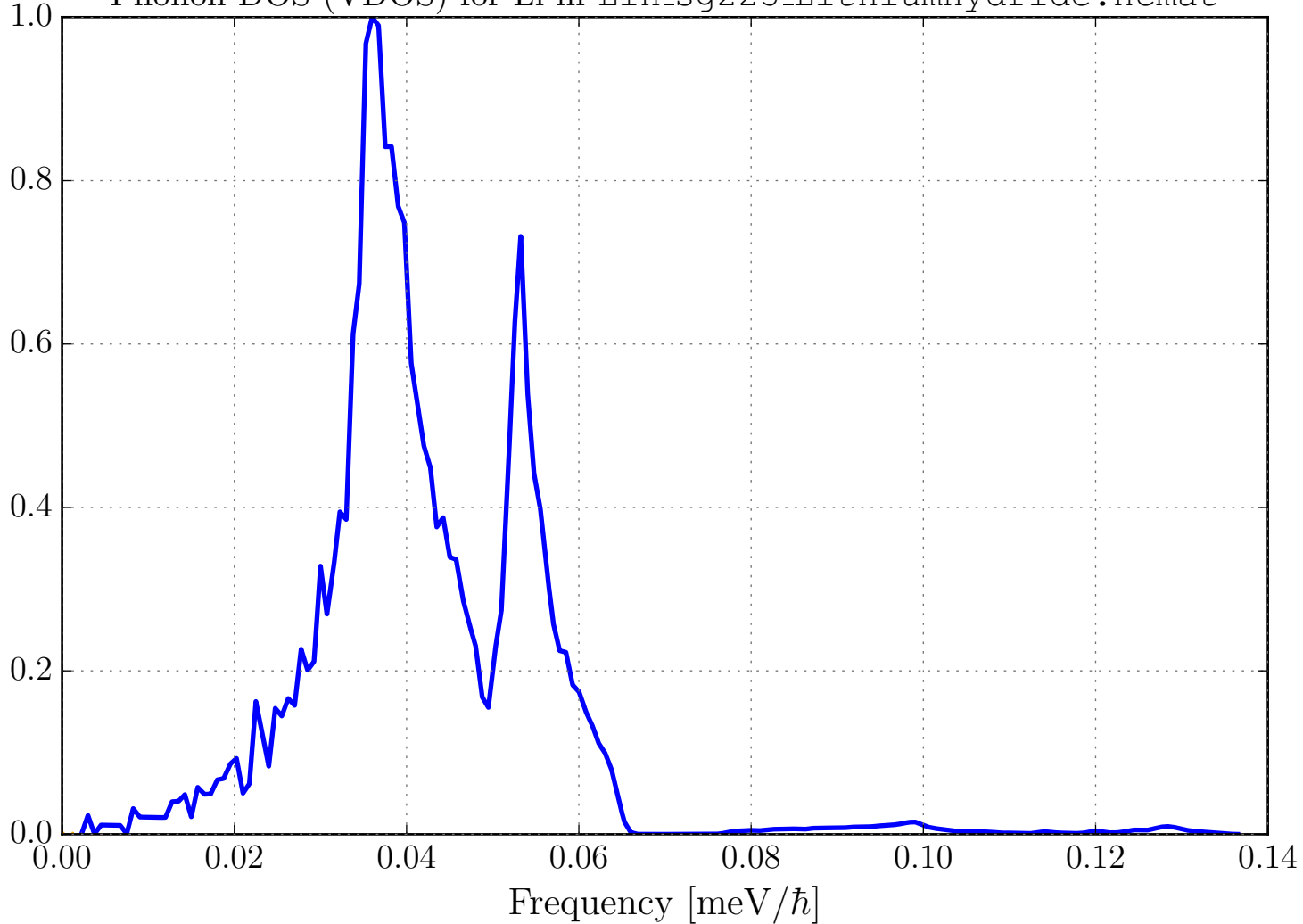
Phonon DOS (VDOS) for Li in LiH_sg225_LithiumHydride.ncmat
