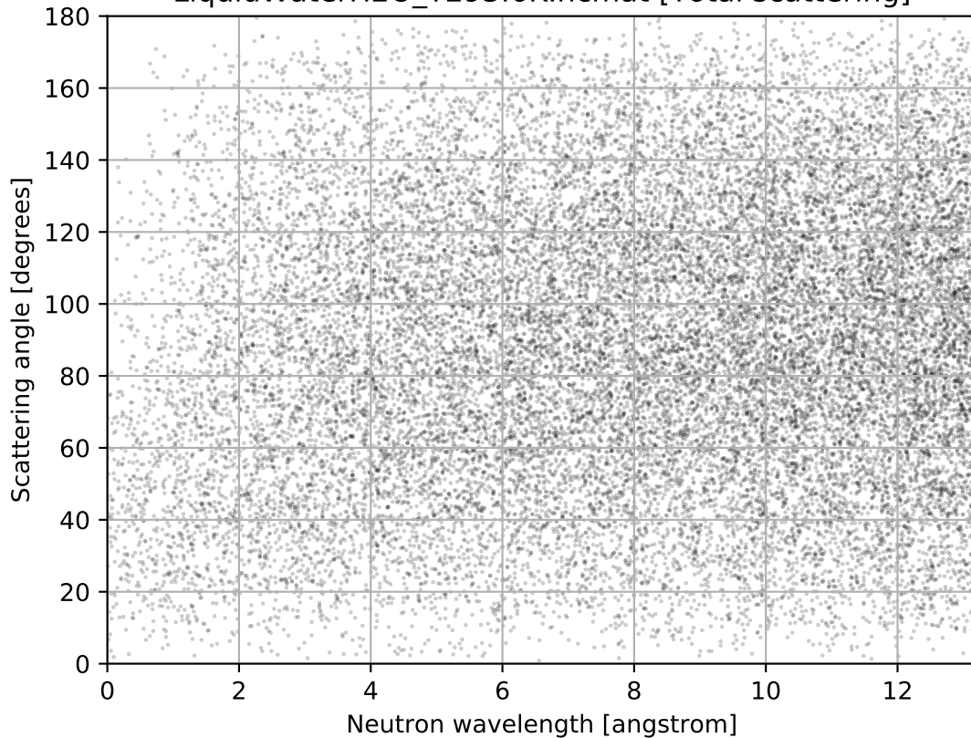
LiquidWaterH2O_T293.6K.ncmat [Total scattering]
