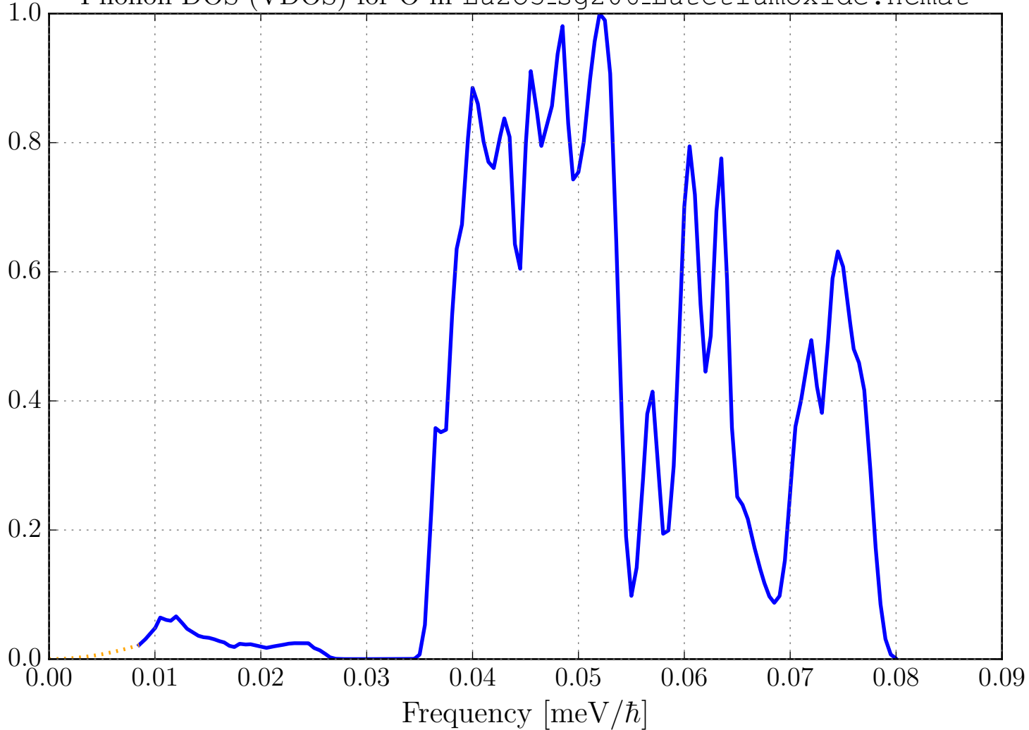
Phonon DOS (VDOS) for O in Lu2O3_sg206_LutetiumOxide.ncmat
