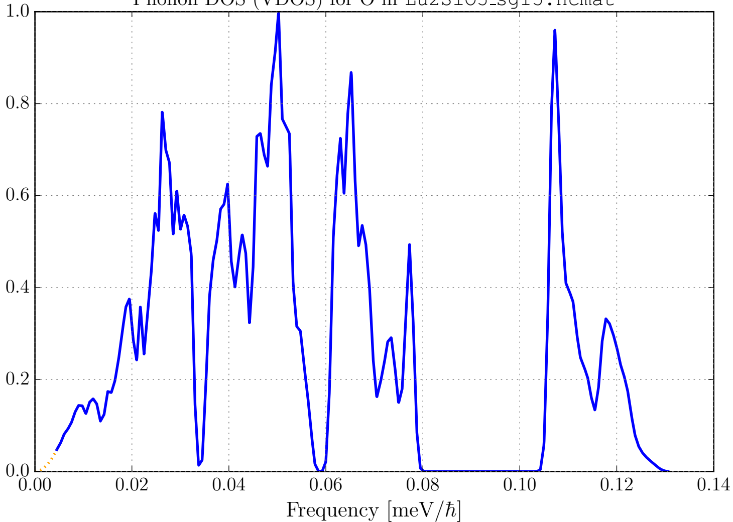
Phonon DOS (VDOS) for O in Lu 2 SiO 5 _sg15.ncmat
