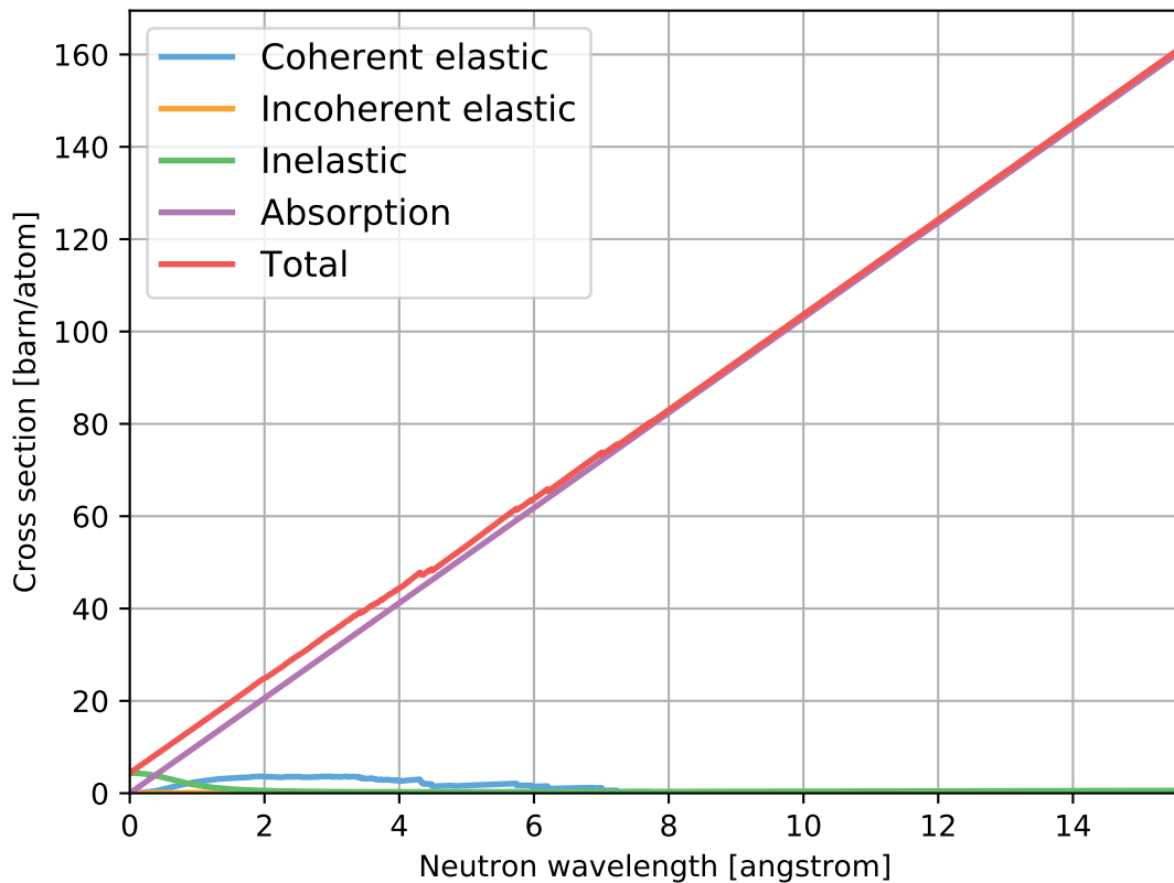
Lu2SiO5_sg15.ncmat [dcutoff=0.3]
