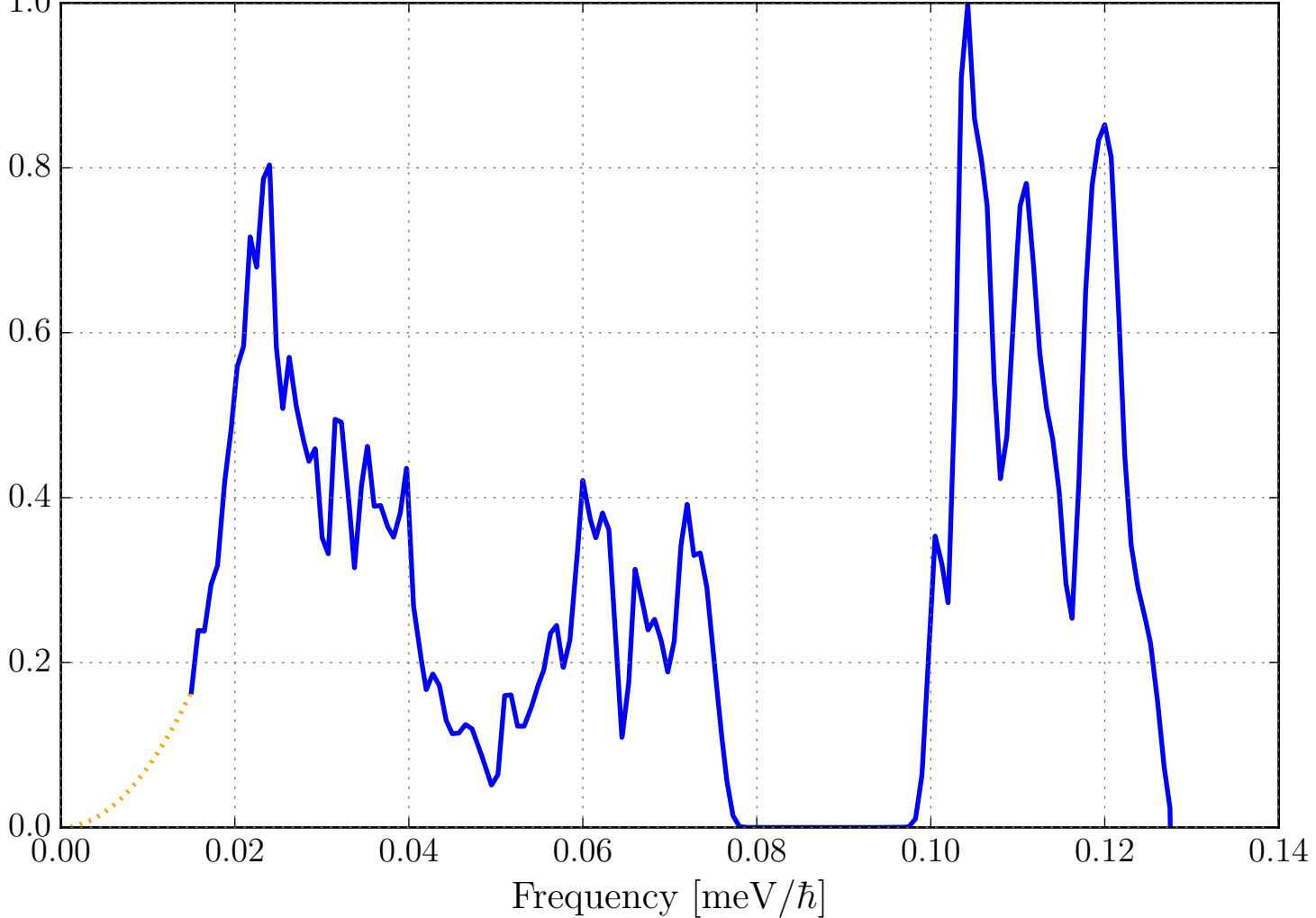
Phonon DOS (VDOS) for Si in Mg 2 SiO 4 _sg62_MagnesiumSilicate.ncmat
