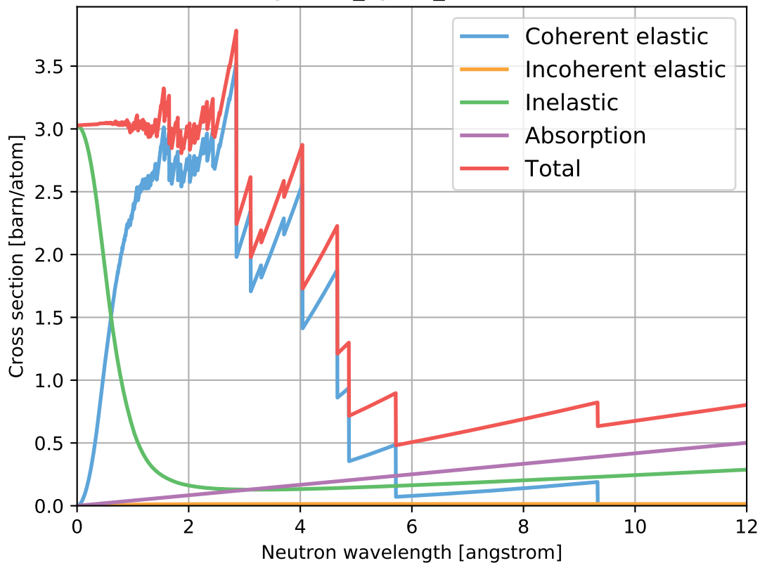
MgAl2O4_sg227_MAS.ncmat
