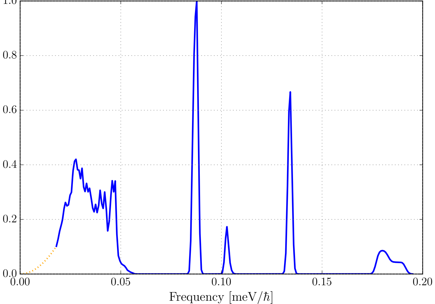
Phonon DOS (VDOS) for O in MgCO3_sg167_MagnesiumCarbonate.ncmat
