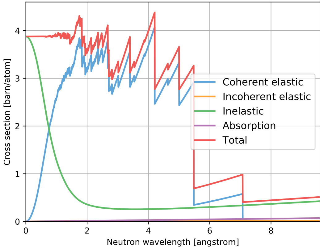
MgCO3_sg167_MagnesiumCarbonate.ncmat
