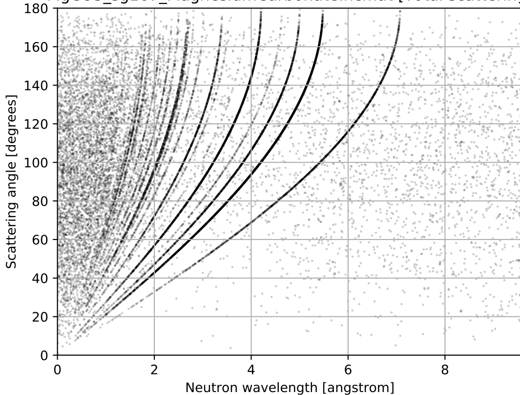
MgCO3_sg167_MagnesiumCarbonate.ncmat [Total scattering]
