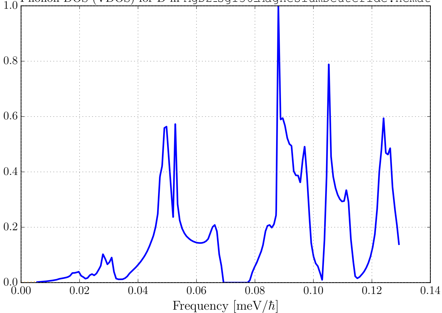
Phonon DOS (VDOS) for D in MgD2_sg136_MagnesiumDeuteride.ncmat
