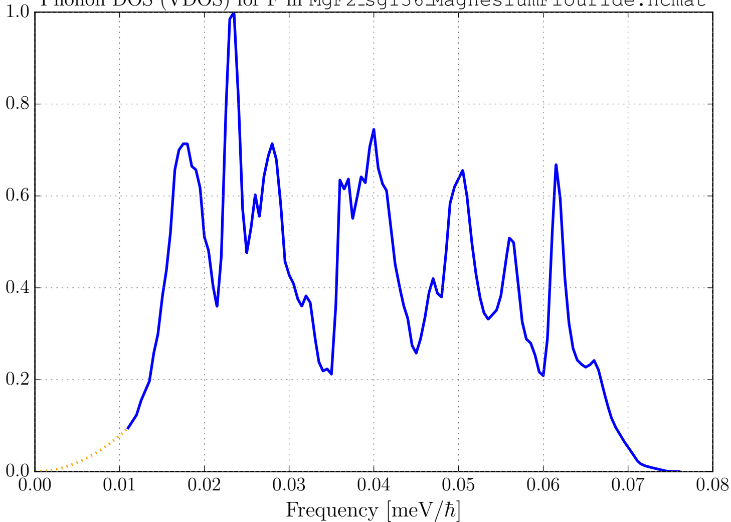
Phonon DOS (VDOS) for F in MgF2_sg136_MagnesiumFlouride.ncmat
