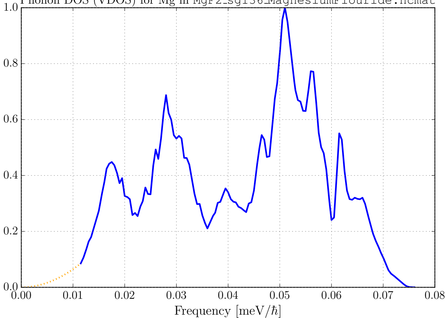
Phonon DOS (VDOS) for Mg in MgF2_sg136_MagnesiumFlouride.ncmat
