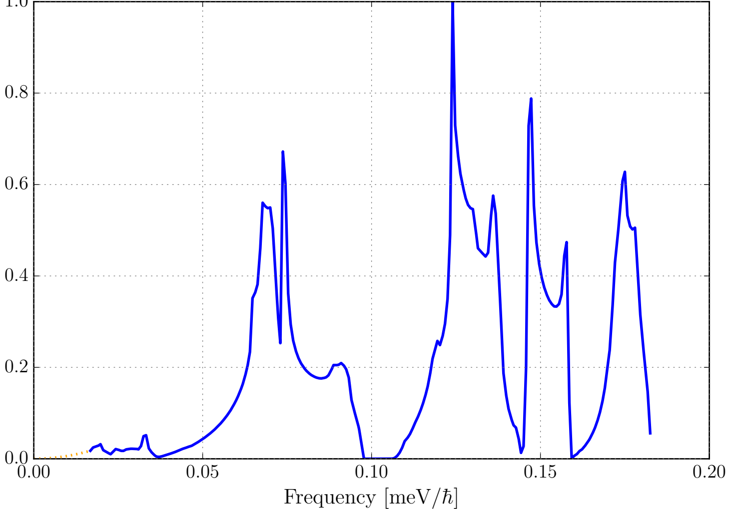
Phonon DOS (VDOS) for H in MgH2_sg136_MagnesiumHydride.ncmat
