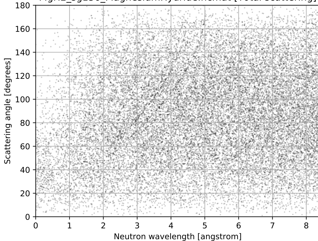
MgH2_sg136_MagnesiumHydride.ncmat [Total scattering]
