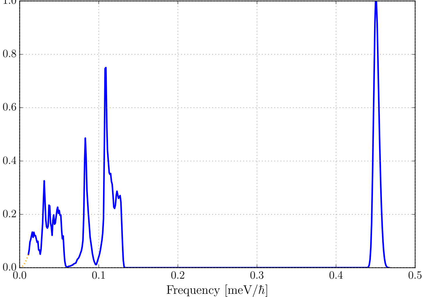
Phonon DOS (VDOS) for H in MgO2H2_sg164_MagnesiumHydroxide.ncmat
