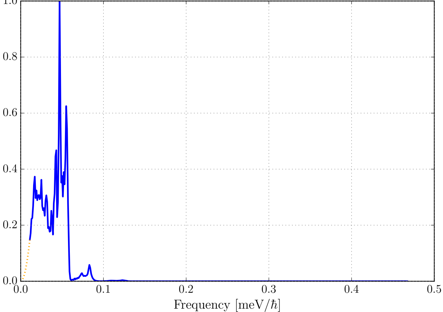
Phonon DOS (VDOS) for Mg in MgO2H2_sg164_MagnesiumHydroxide.ncmat
