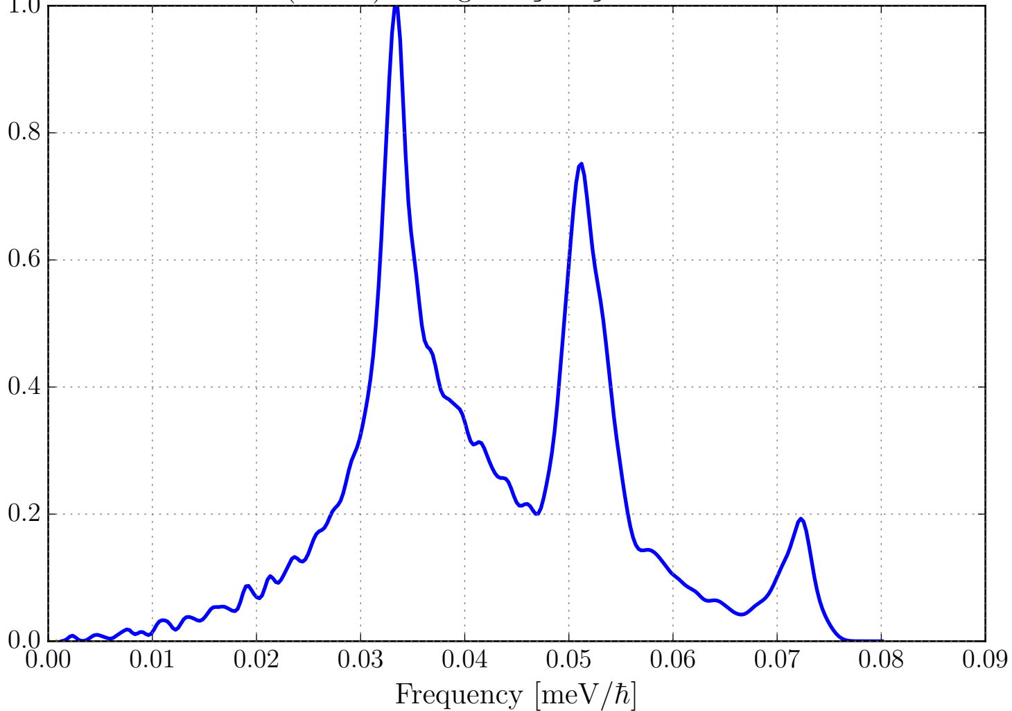
Phonon DOS (VDOS) for Mg in MgO_sg225_Periclase.ncmat
