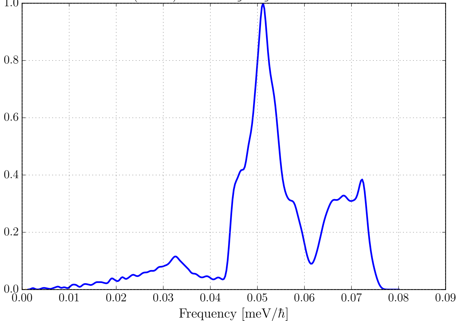
Phonon DOS (VDOS) for O in MgO_sg225_Periclase.ncmat
