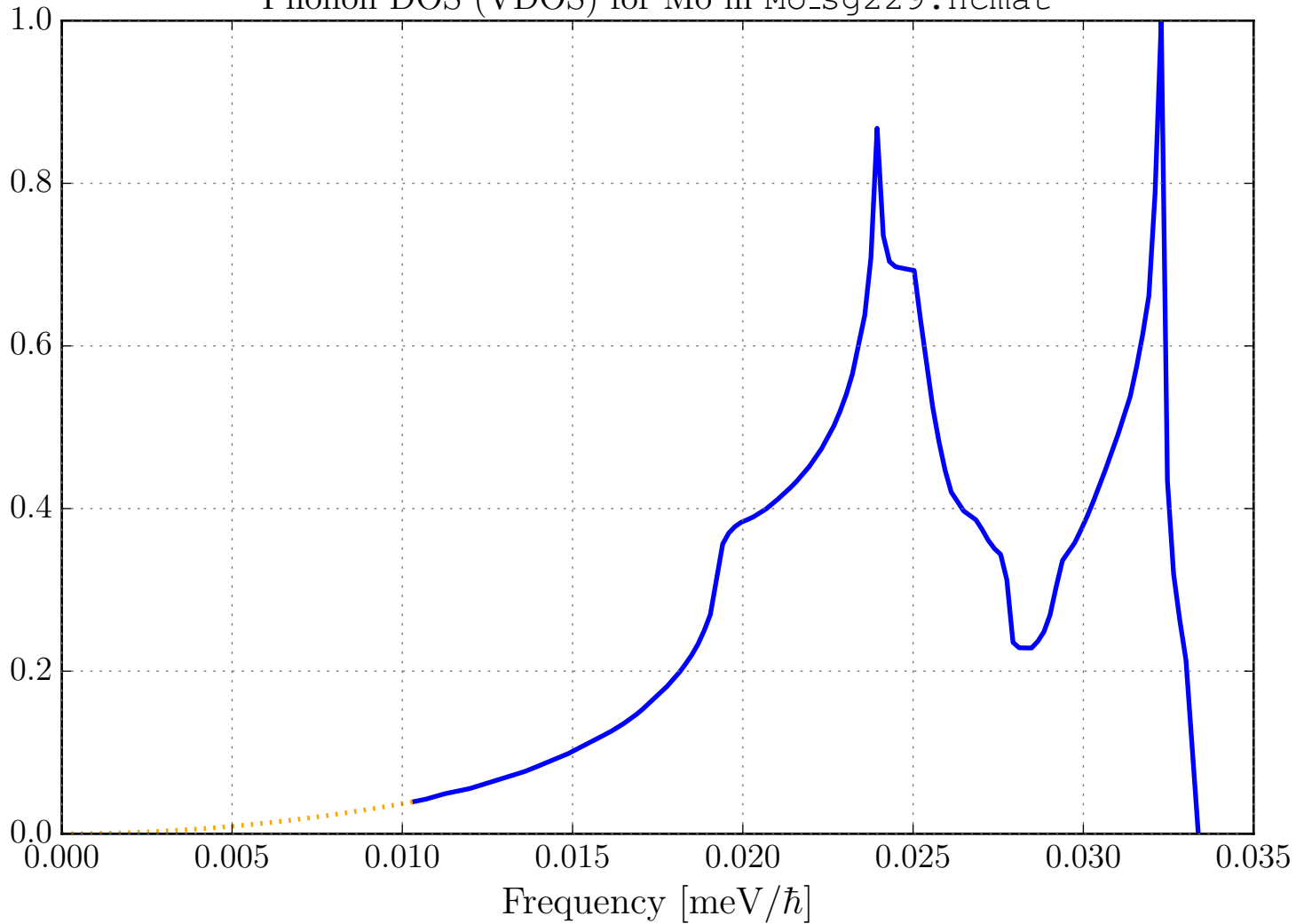
Phonon DOS (VDOS) for Mo in Mo_sg229.ncmat
