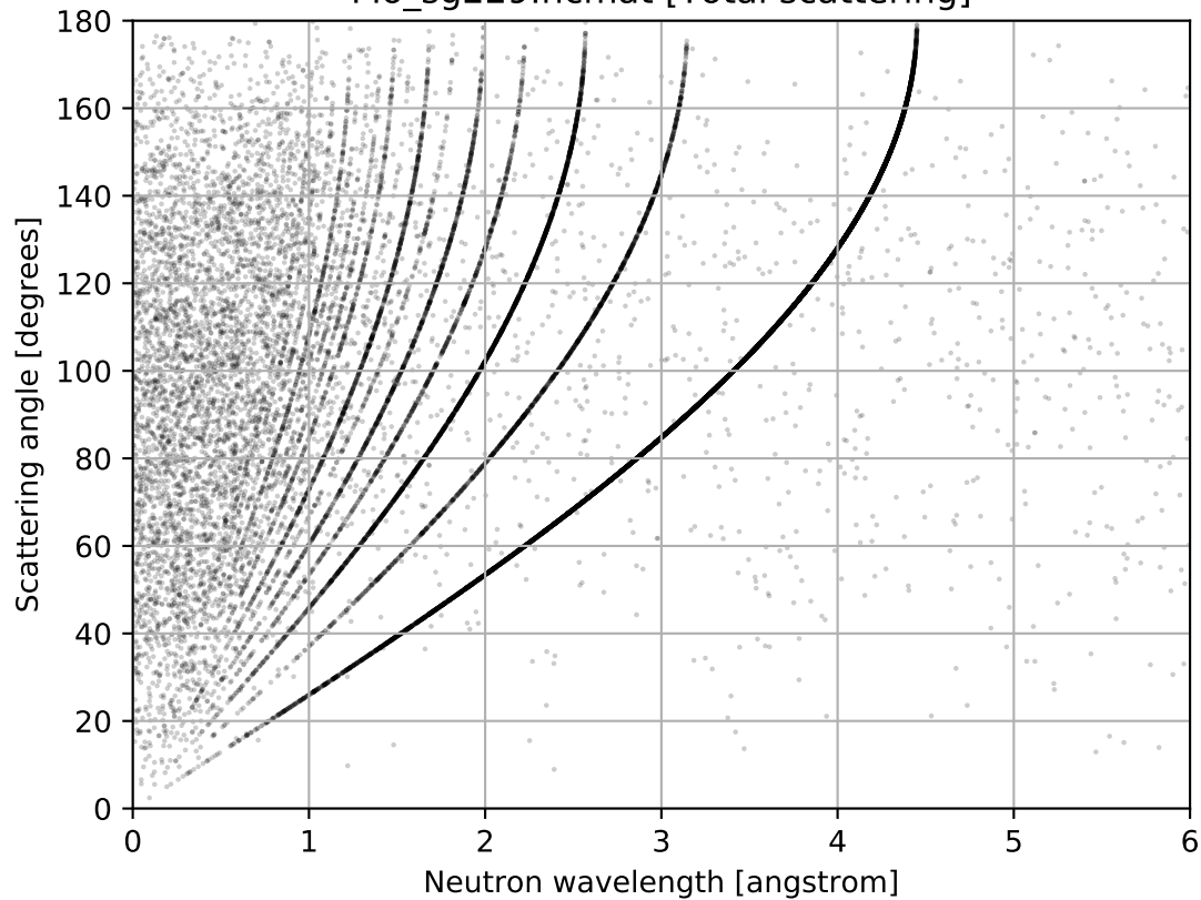
Mo_sg229.ncmat [Total scattering]
