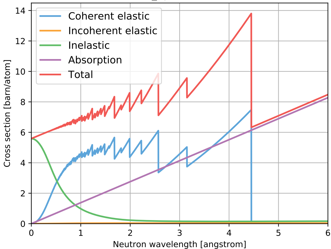
Mo_sg229.ncmat
