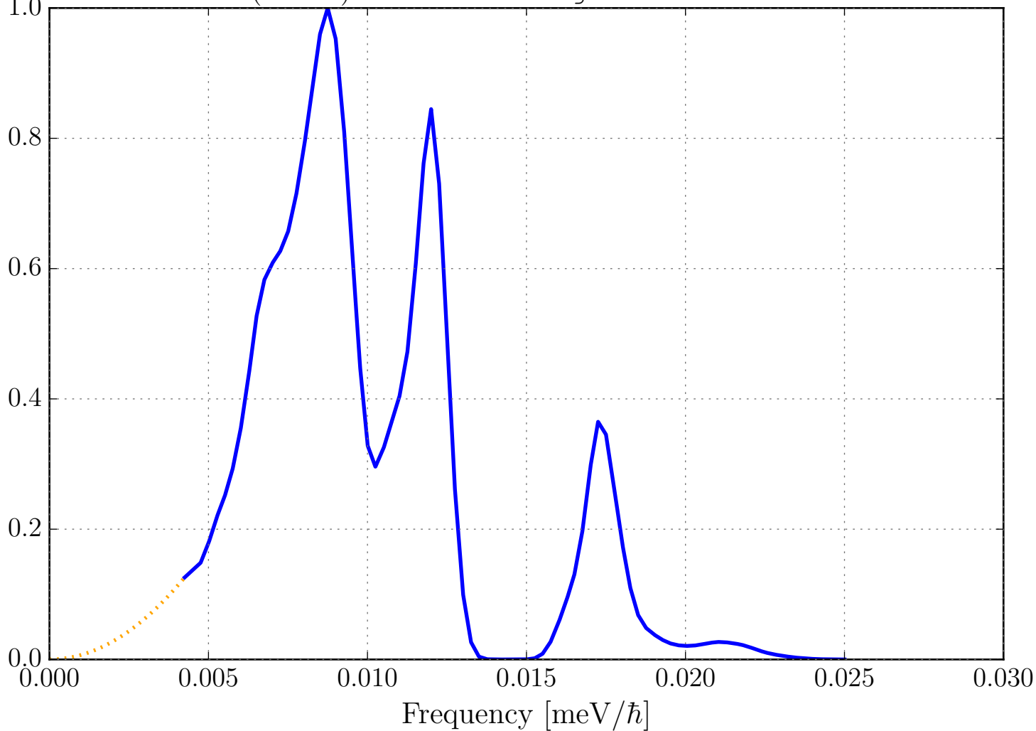
Phonon DOS (VDOS) for Br in NaBr_sg225_SodiumBromide.ncmat
