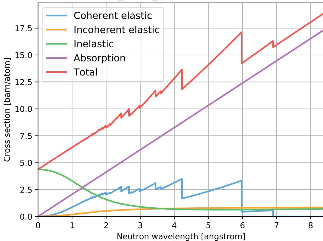
NaBr_sg225_SodiumBromide.ncmat
