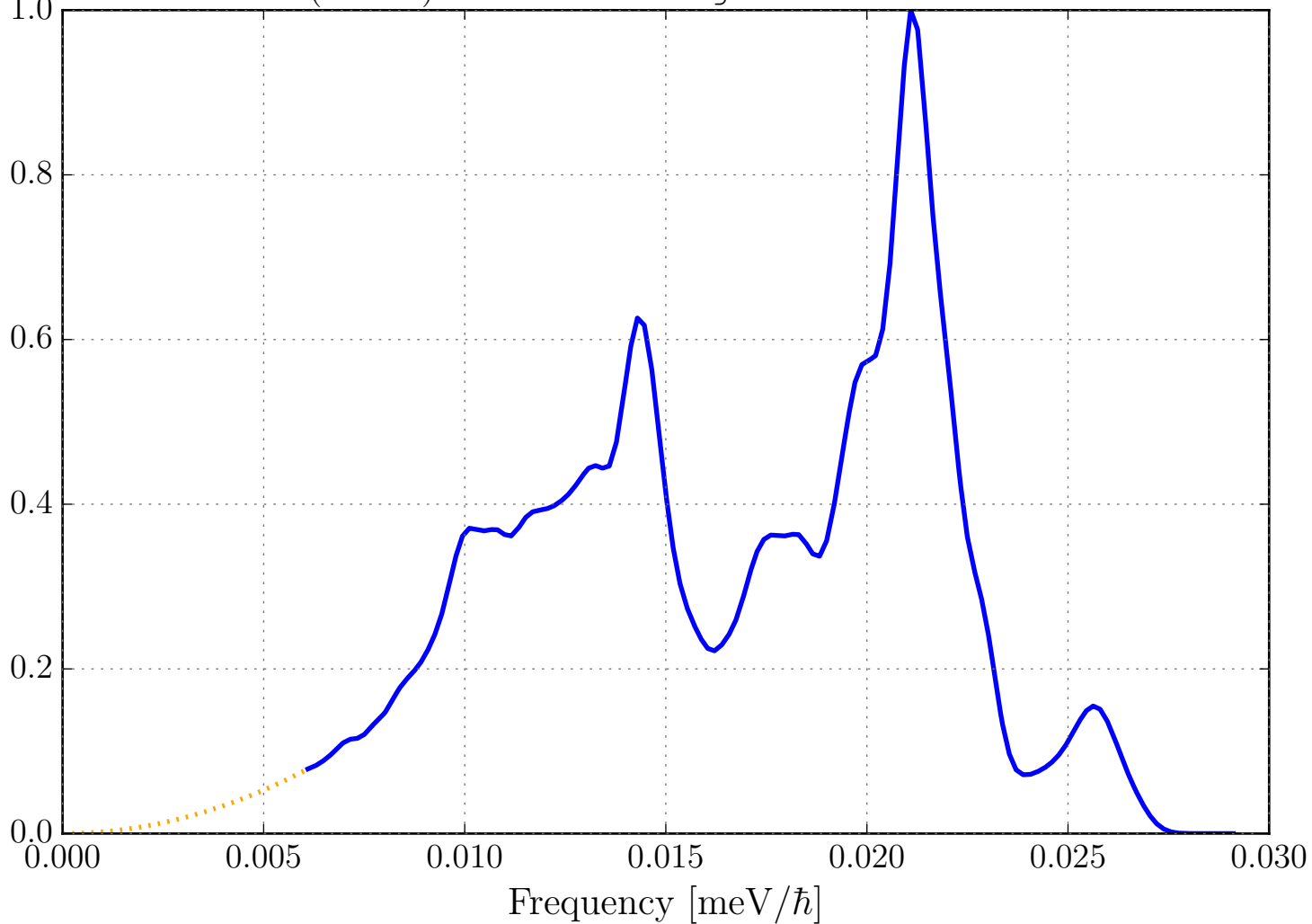
Phonon DOS (VDOS) for Cl in NaCl_sg225_SodiumChloride.ncmat
