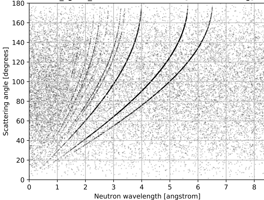
NaCl_sg225_SodiumChloride.ncmat [Total scattering]
